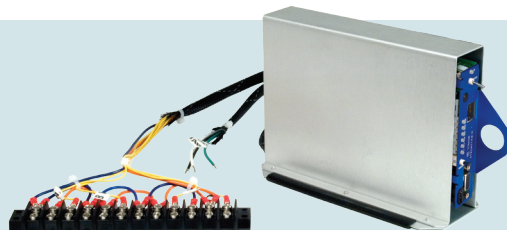
1881 Card Cage and Harness
