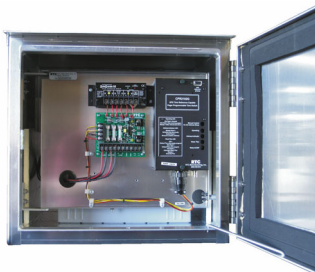
Compact cabinet holds time switch, solar regulator, flasher/fuse board and battery.
